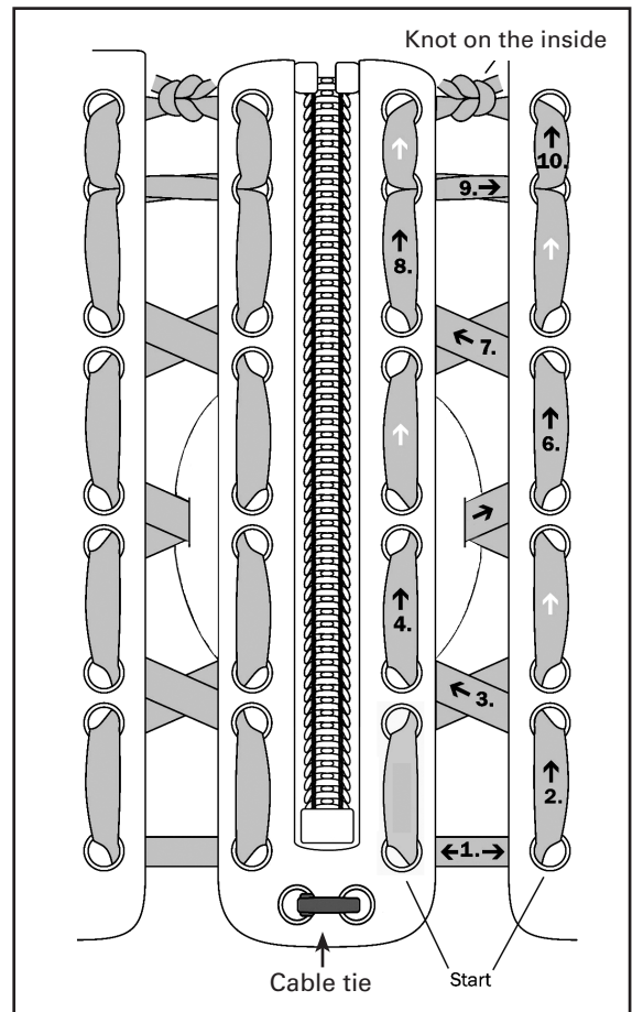
FIG. 2 Zipper Assembly
